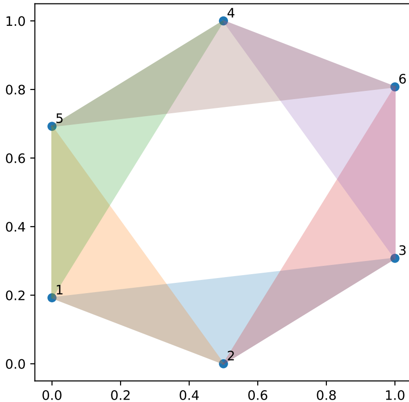
The 6 minimal area triangles for n=6
